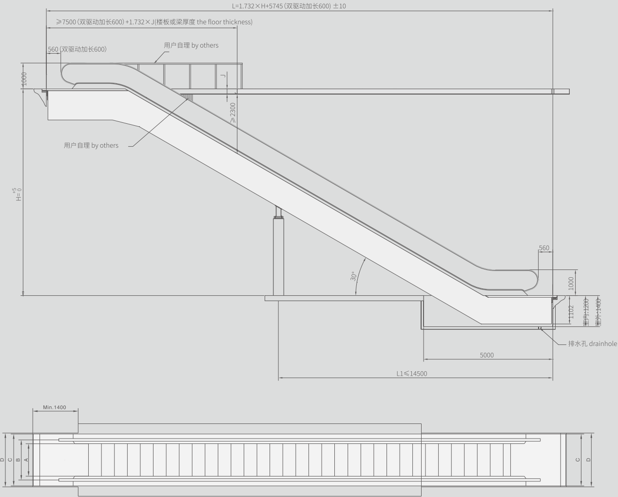
土建示意图仅供参考 The schematic drawing of civil work is for reference only
