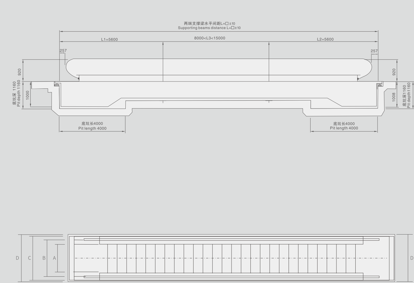
土建示意图仅供参考 The schematic drawing of civil work is for reference only
